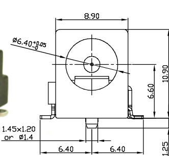
Part No. FC68149S
