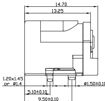
Part No. FC68149S
