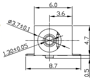
Part No. FC68145S Taped FC68145ST
