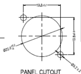
PANEL CUTOUT
