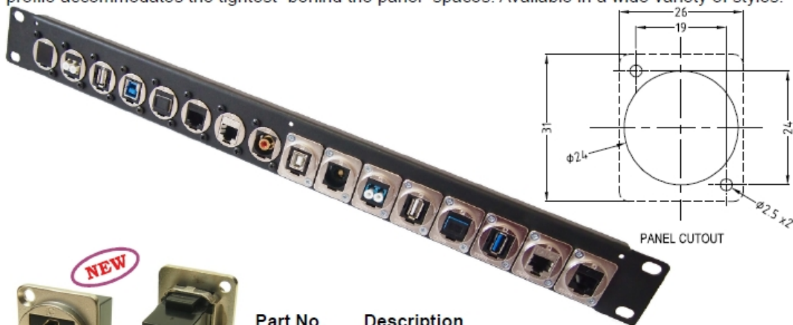
Part No. Description CP30200GM HDMI A Female to HDMI A, Gold Plated, CSK hole.
