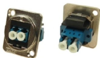
Part No. Description CP30213M LC Duplex SM adaptor, Nickel Plated, CSK Hole
